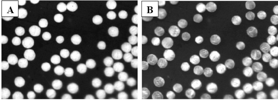
Figure 19 Cross-sectional view of commercial pitch based carbon fiber P25 under (A) normal light and (B) polarized light
