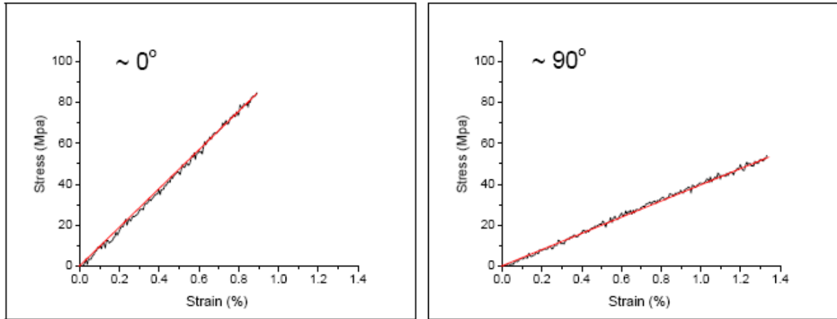
Figure 59 Typical stress-strain curves of carbon fiber composites at \sim 0^\circ and \sim 90^\circ
