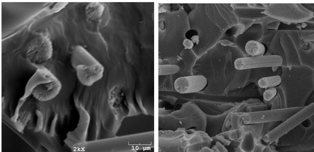
Figure 56 SEM micrograph of fracture surface of carbon fiber composite showing good and bad bondings
