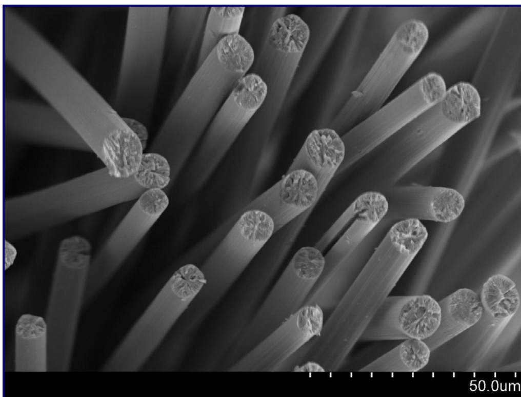
Figure 24 SEM image of pitch-based carbon fibers processed at 1550 °C
