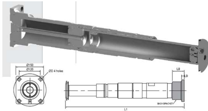
(a) Back mounted Oleo 110 Series Industrial Energy Absorber [21]
