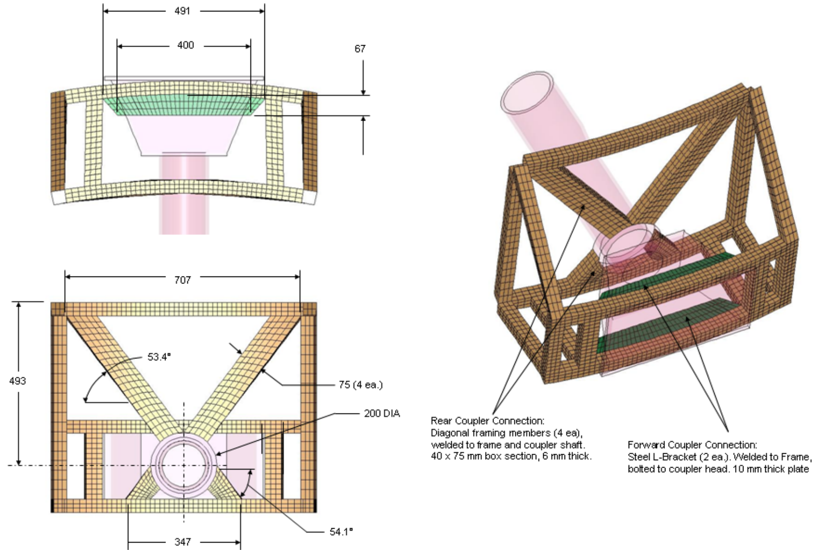
Figure 49. Detail: Connection of center frame to coupler.
