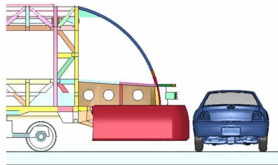
(b) Less aggressive lowered profile
