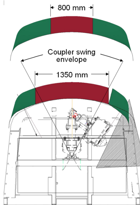
Figure 29. Plan view of segmented bumper notionally attached to the front end of an S70 LRV with swinging coupler.
