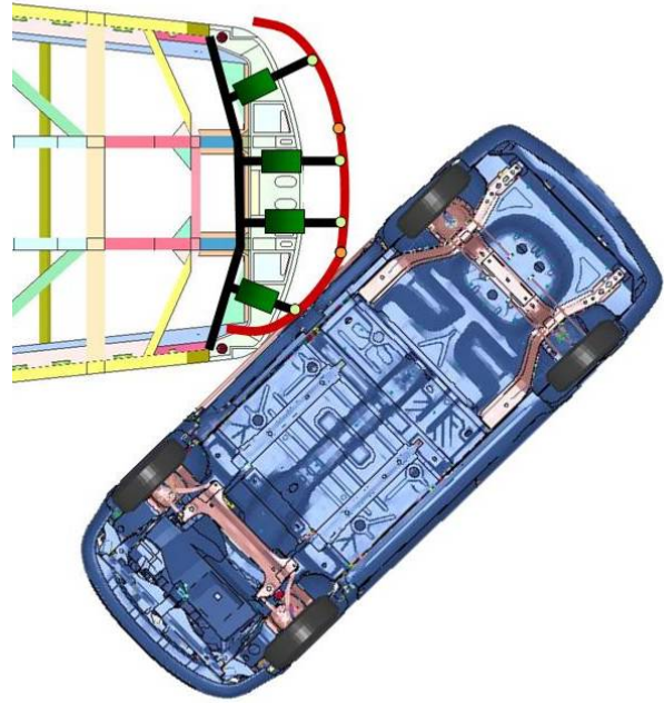
(b) 45 degree impact
