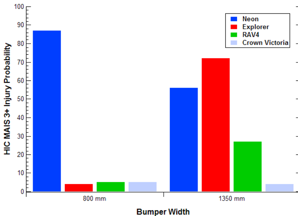
Figure 32. Probability of 'Serious' (AIS 3+) head injury from 48.2 km/hr (30 mph), 45 degree impacts as a function of bumper width.
