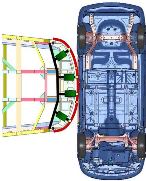
(a) 90 degree impact
