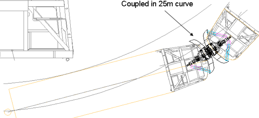
Figure 42. Segmented bumper retrofit conceptual design functionality during coupled operation.
