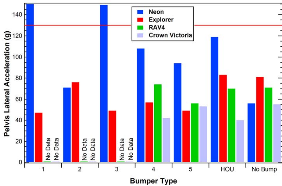
Figure 24. Pelvis acceleration from 32.2 km/hr (20 mph), 90 degree impacts.
