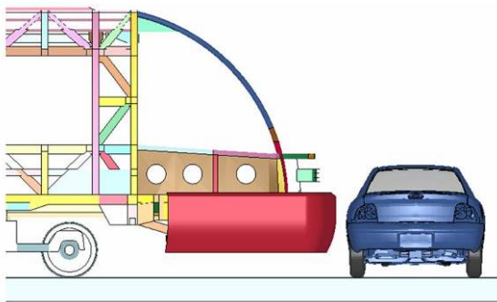
(a) Existing bumper profile
