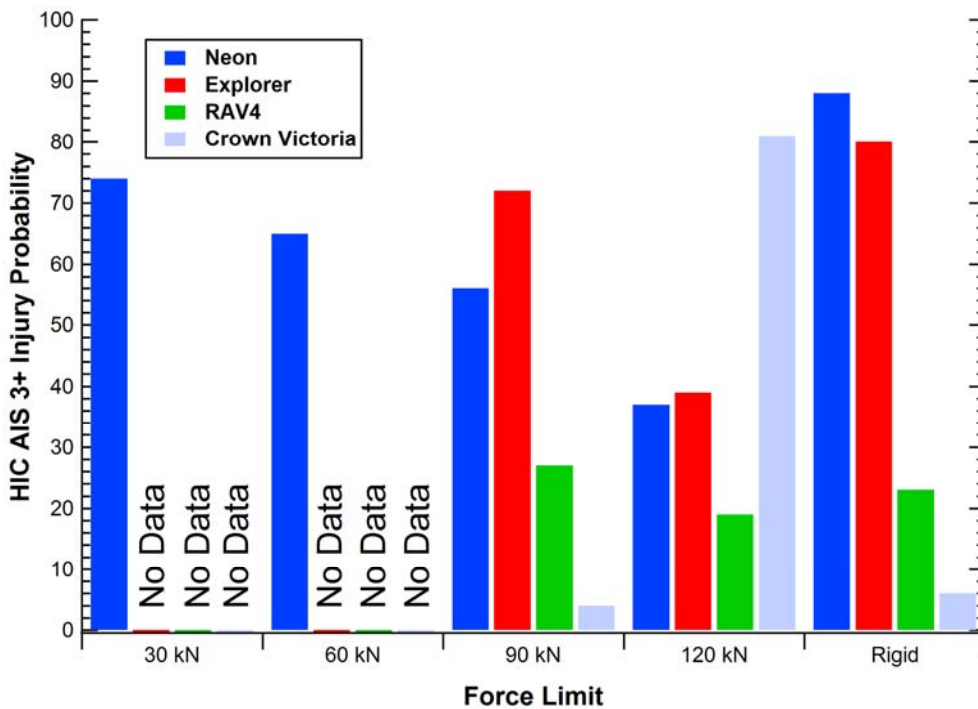
Figure 35. Probability of 'Serious' (AIS 3+) head injury from 48.2 km/hr (30 mph), 45 degree impacts as a function of energy absorber force limit.
