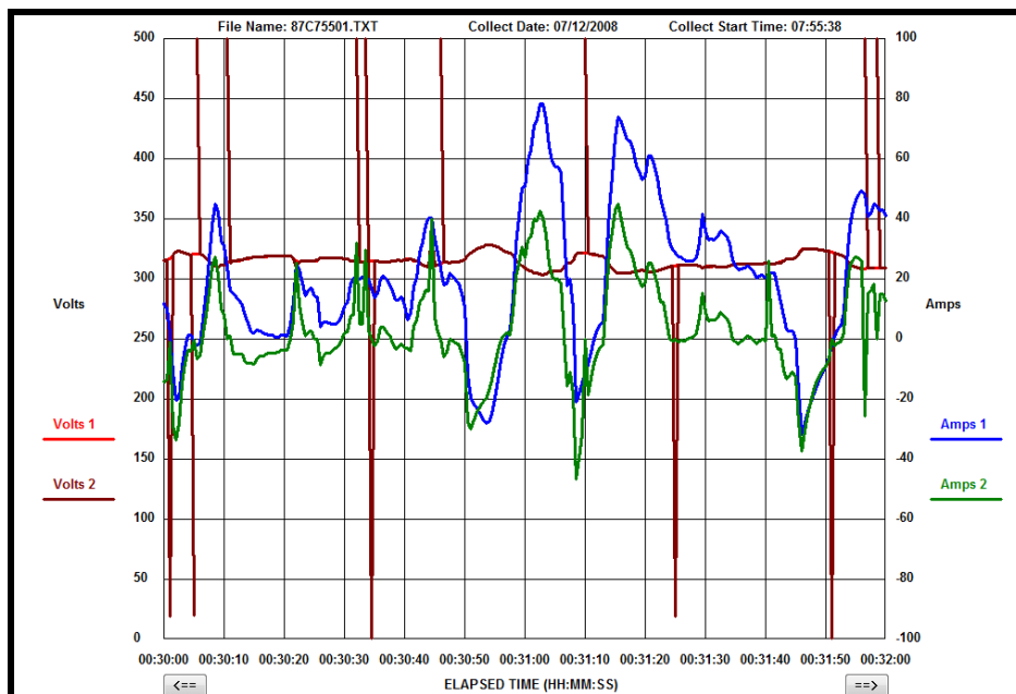
Figure 21. Voltage Spikes on String 2, EV19; 2-min Window
