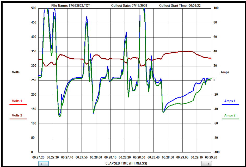
Figure 22. Driving Profile, Emory Bus #802; 2-min Window
