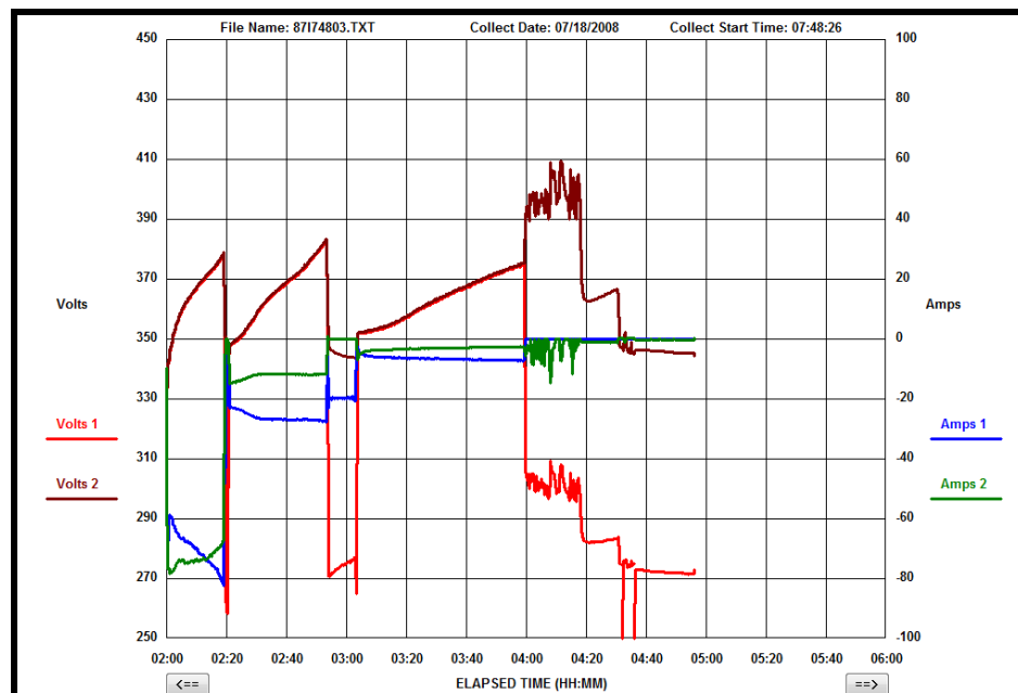
Figure 20. Emory #802 Charge Profile
