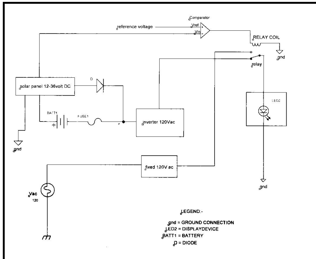
Figure 16. Circuit Design for Dual Power Supply to DMS
