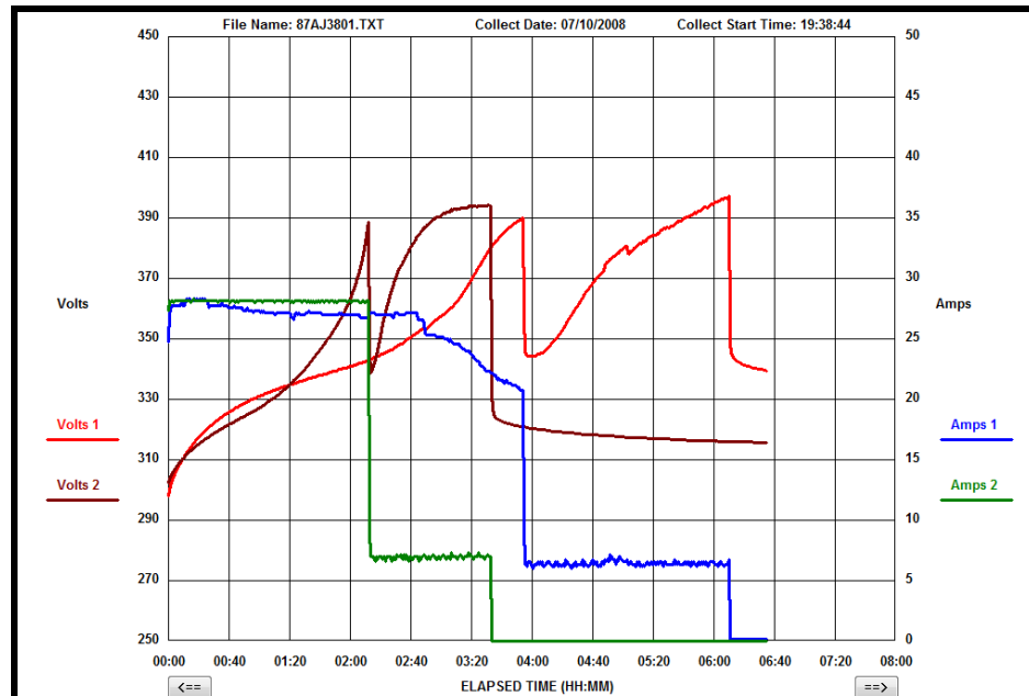
Figure 19. EV19 Recharge Profile
