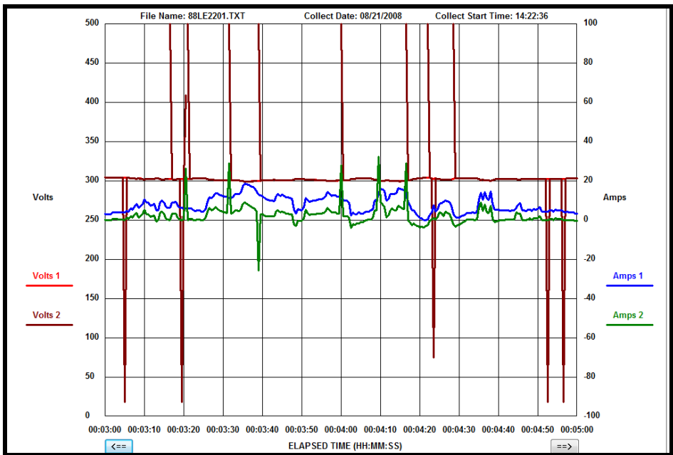
Figure 23. Voltage Spikes on String 2, EV19; Replacement Battery Set
