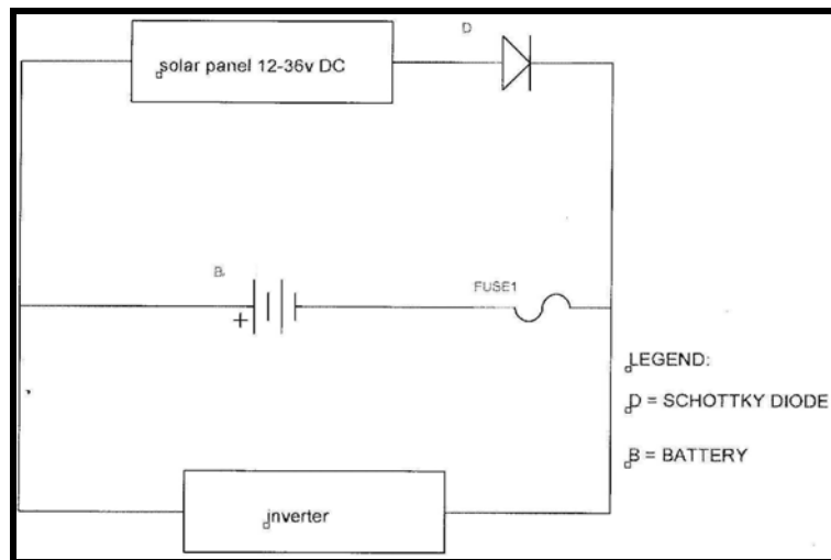
Figure 17. Circuit Design for the Battery Regulator
